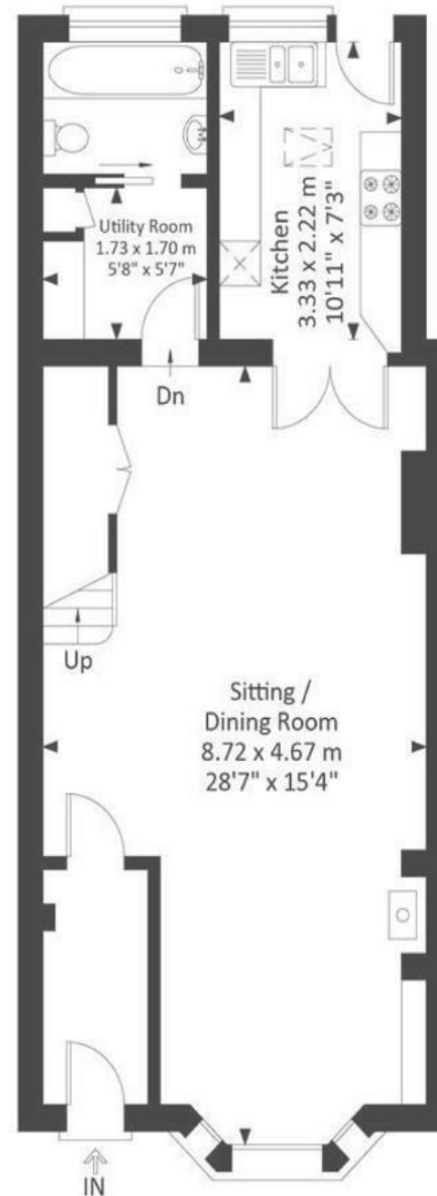
Ground Floor
